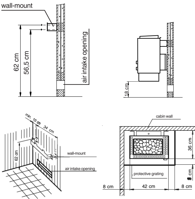
connection diagram for 7,5 kW oven (with 6 kW 3 tubular heating elements with 2000 W each)
