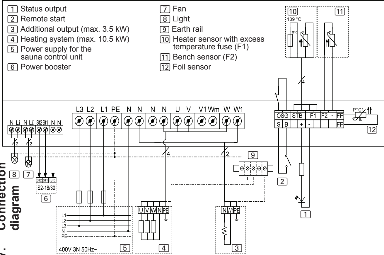
Fig. 4 Connection diagram
