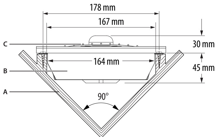
Installation in the cabin corner
