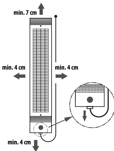
Vitae Protect+ - minimum distances from combustibile materials. Cable connection downwards.
