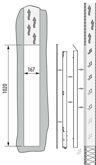
Installation opening and wall structure
