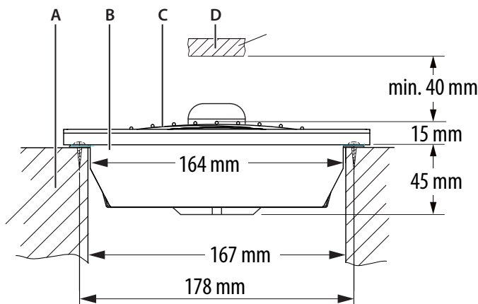
Installation in the cabin wall
